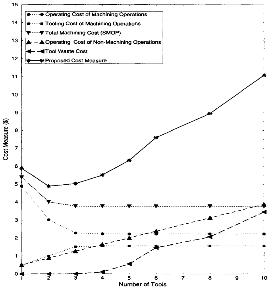
Fig. 2. The detailed analysis of cost measure for operation (12, 1).
