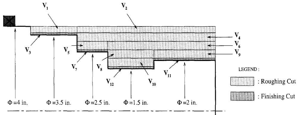
Fig. 1. Machinable volume presentation.
